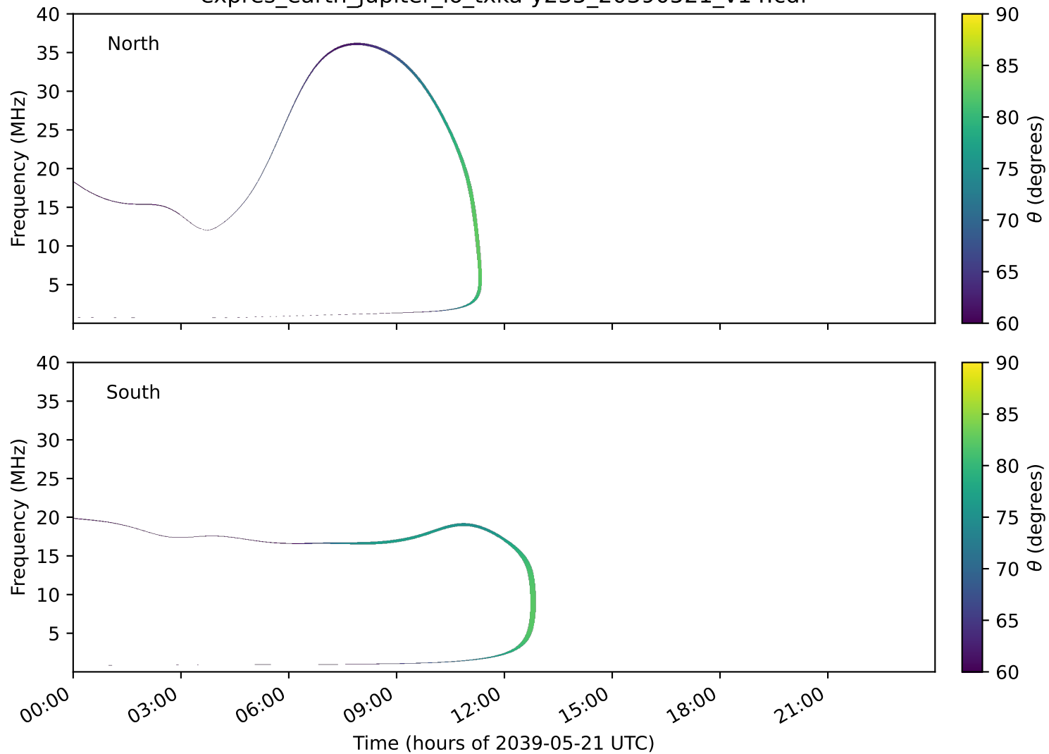
expres_earth_jupiter_io_txka-y235_20390521_v14.cdf
