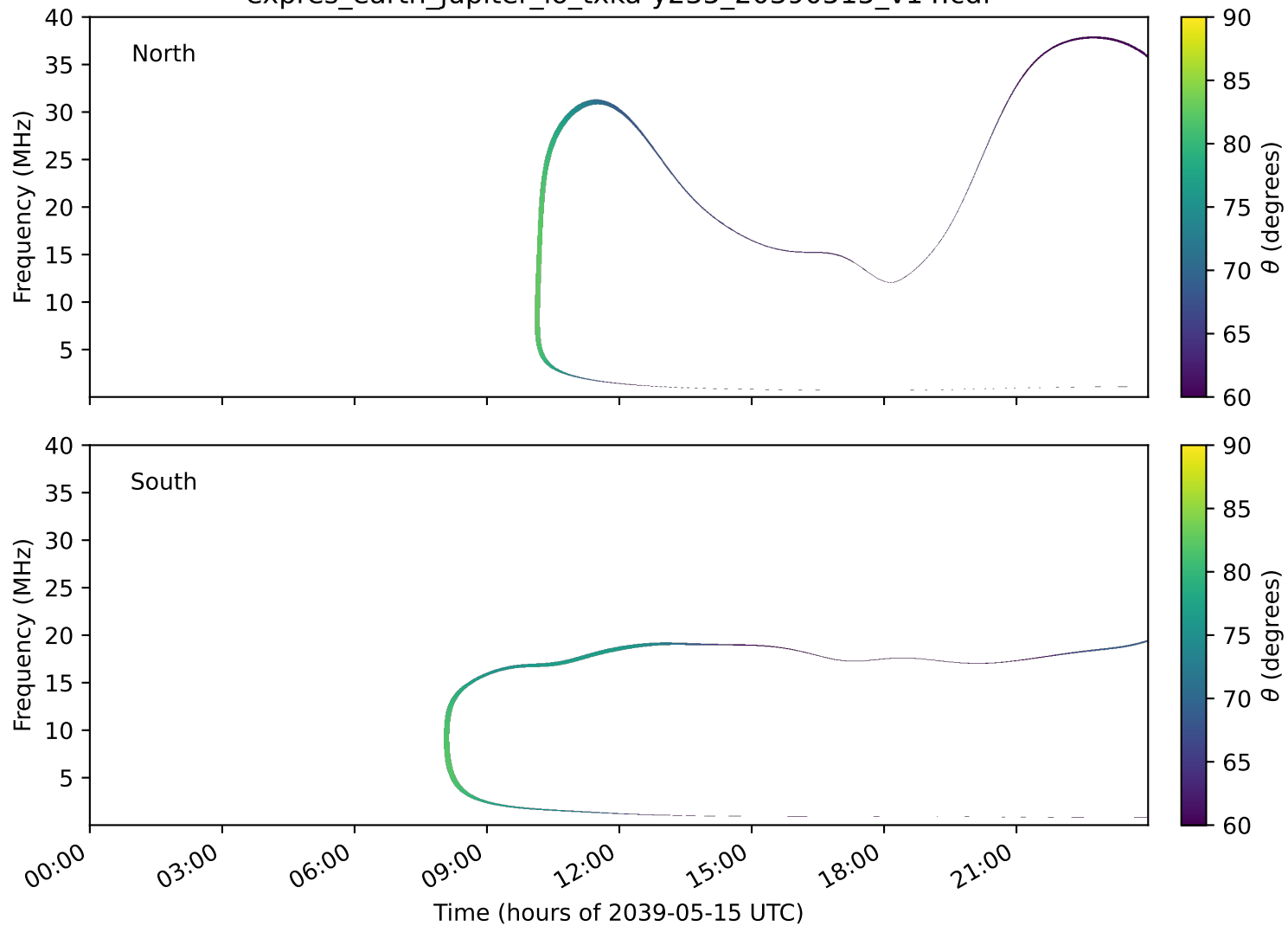
expres_earth_jupiter_io_txka-y235_20390515_v14.cdf
