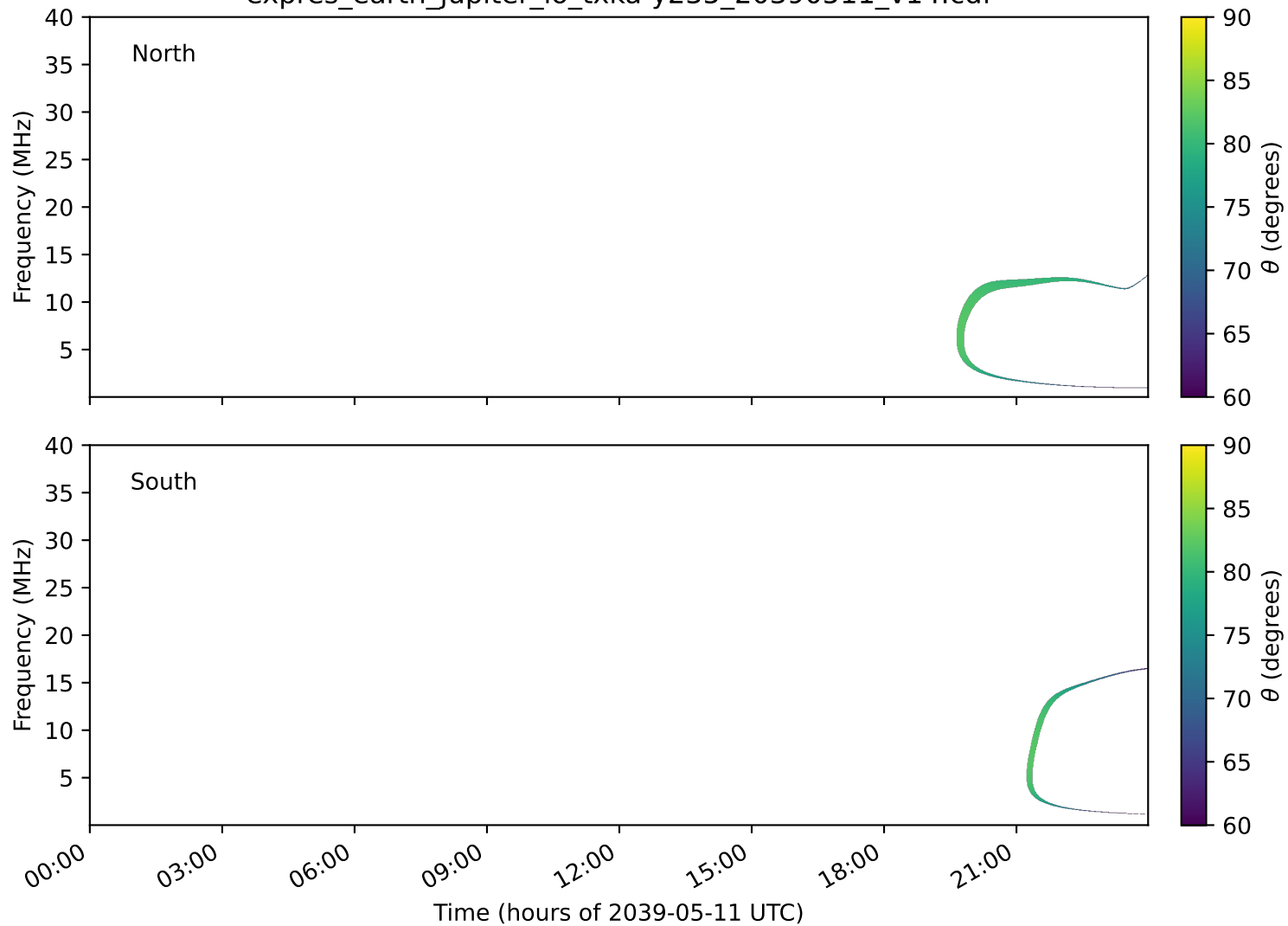
expres_earth_jupiter_io_txka-y235_20390511_v14.cdf
