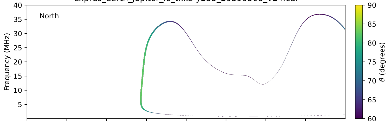
expres_earth_jupiter_io_txka-y235_20390508_v14.cdf
