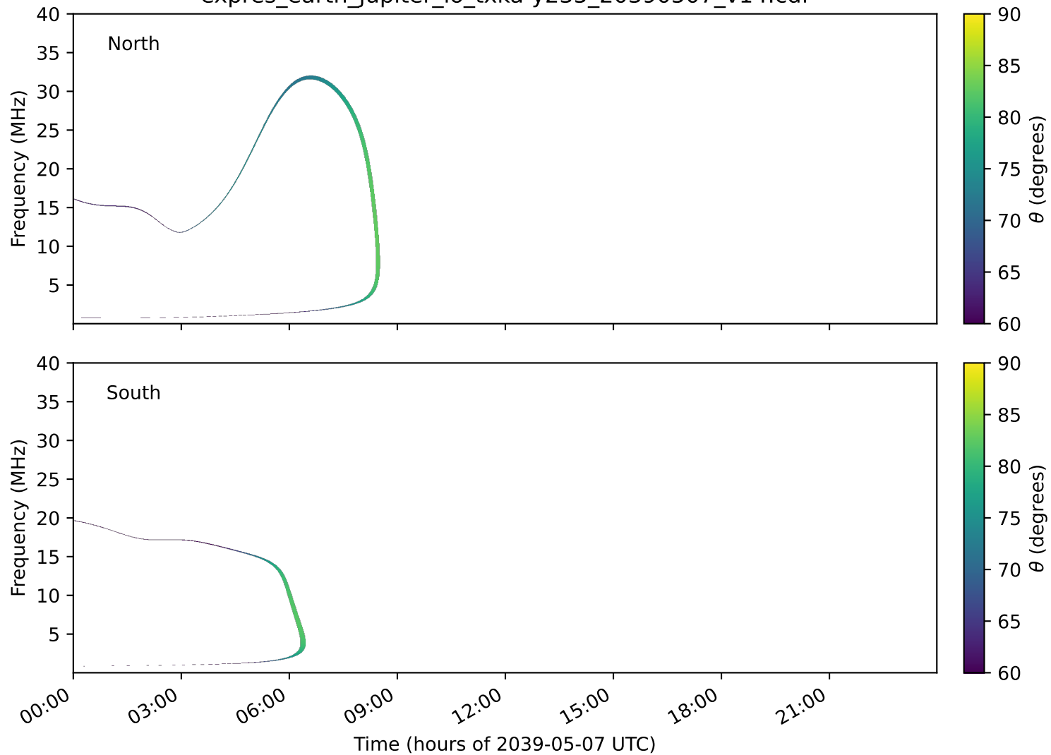
expres_earth_jupiter_io_txka-y235_20390507_v14.cdf
