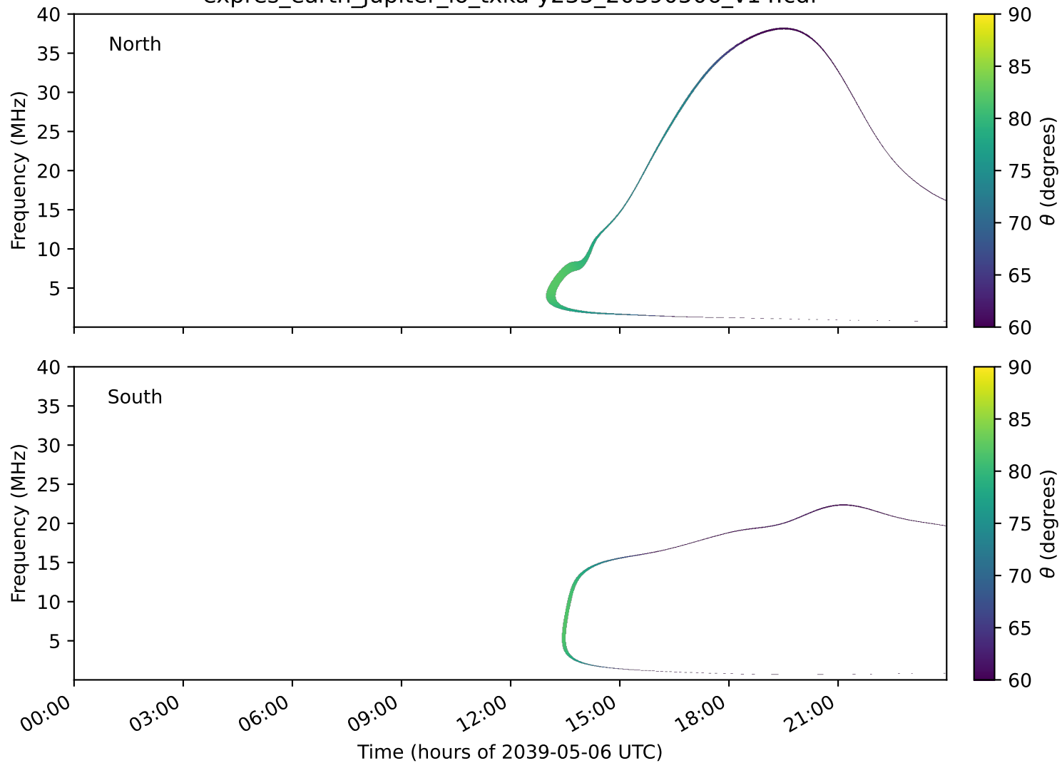
expres_earth_jupiter_io_txka-y235_20390506_v14.cdf
