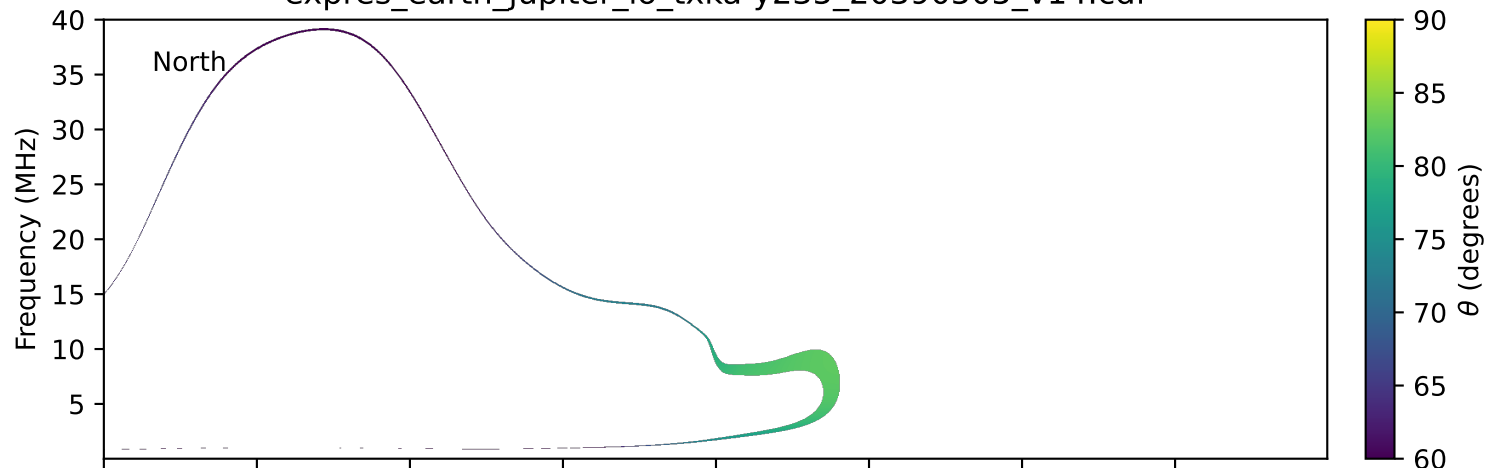
expres_earth_jupiter_io_txka-y235_20390505_v14.cdf
