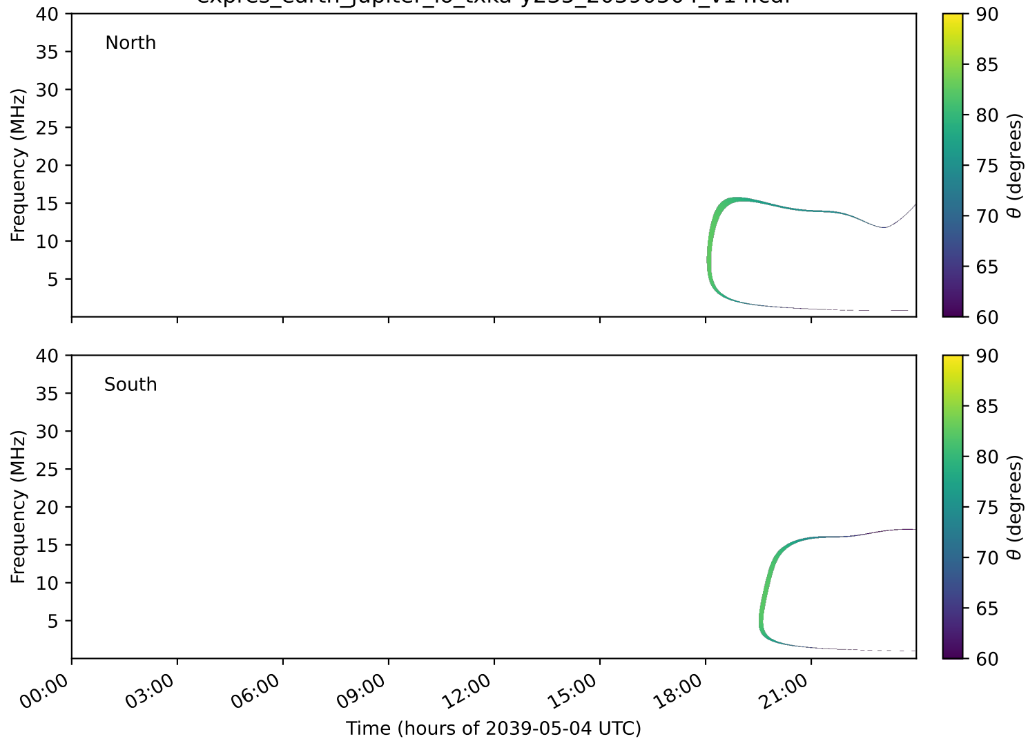
expres_earth_jupiter_io_txka-y235_20390504_v14.cdf
