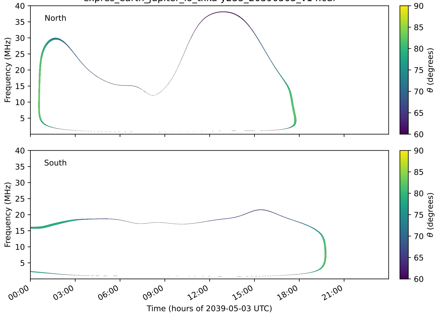
expres_earth_jupiter_io_txka-y235_20390503_v14.cdf
