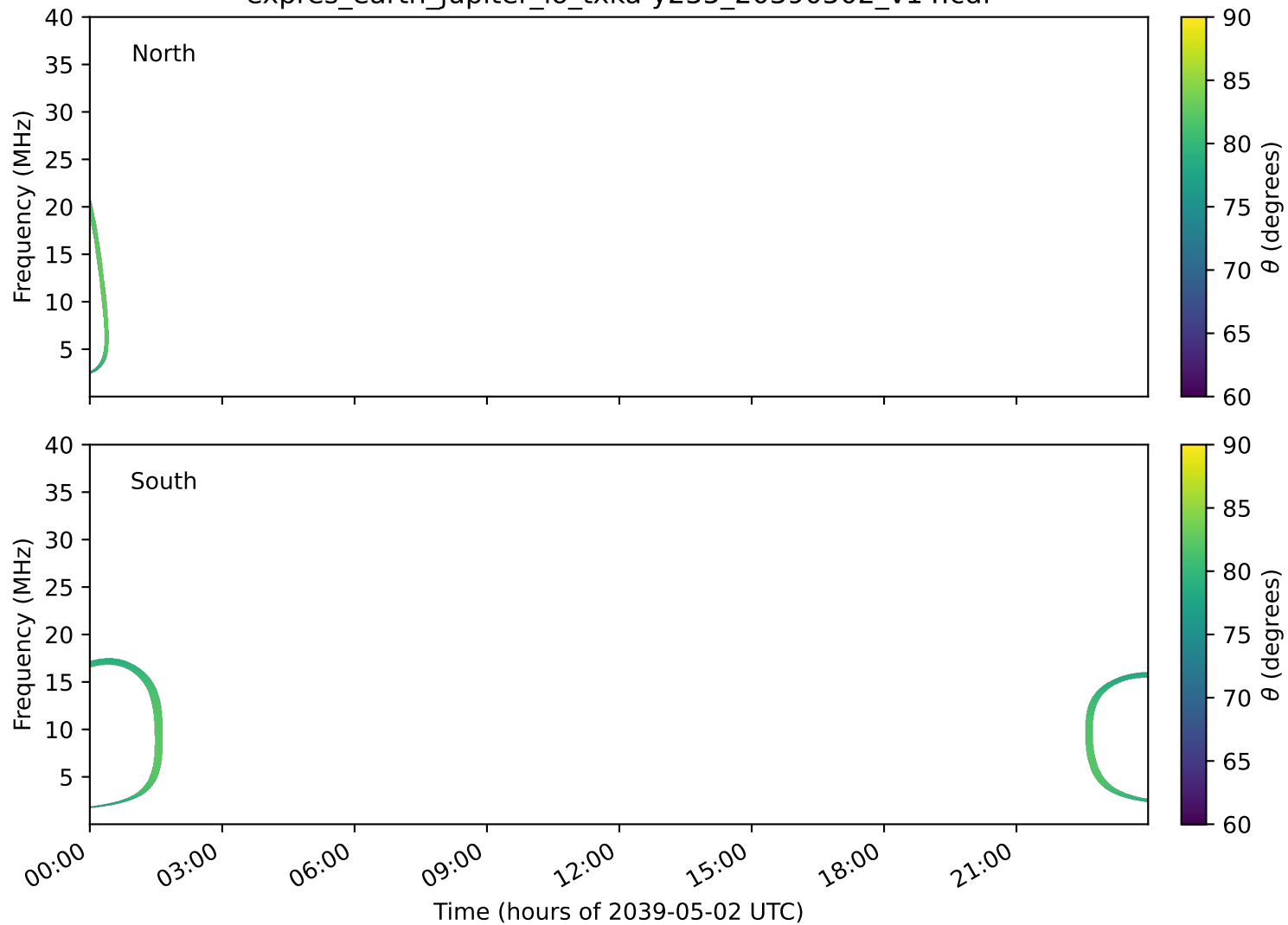
expres_earth_jupiter_io_txka-y235_20390502_v14.cdf
