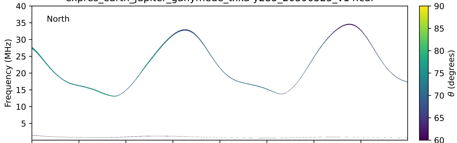
expres_earth_jupiter_ganymede_txka-y235_20390525_v14.cdf
