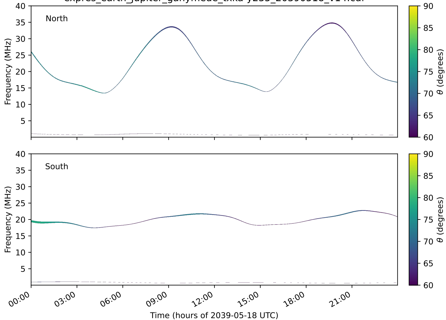
expres_earth_jupiter_ganymede_txka-y235_20390518_v14.cdf
