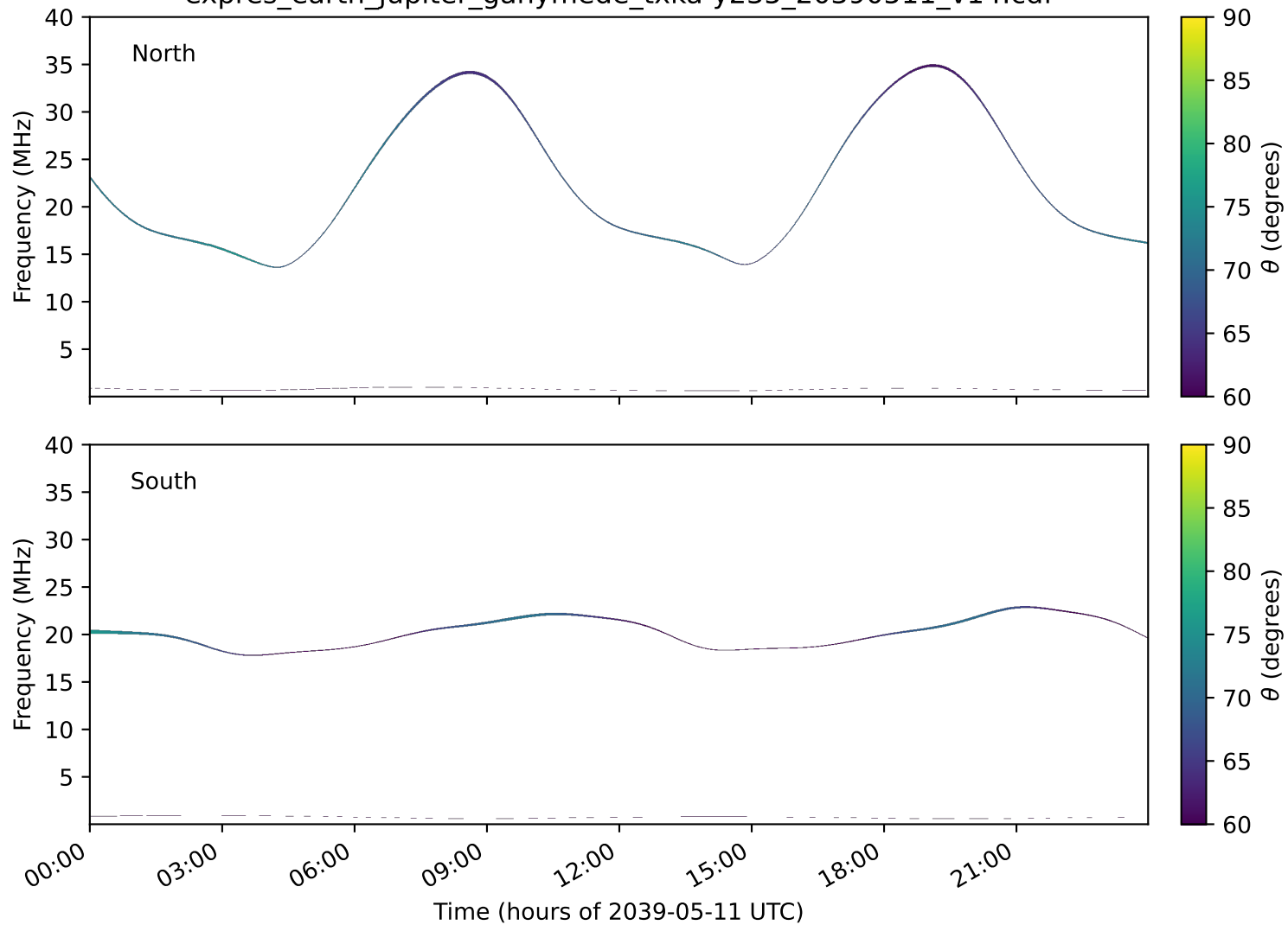
expres_earth_jupiter_ganymede_txka-y235_20390511_v14.cdf
