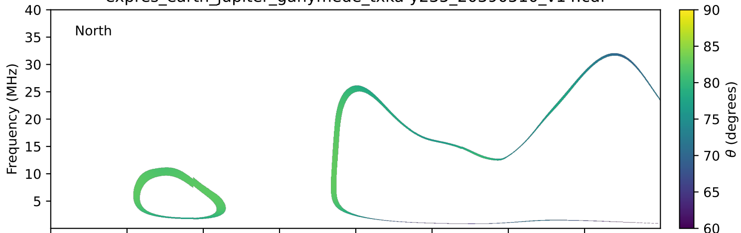
expres_earth_jupiter_ganymede_txka-y235_20390510_v14.cdf
