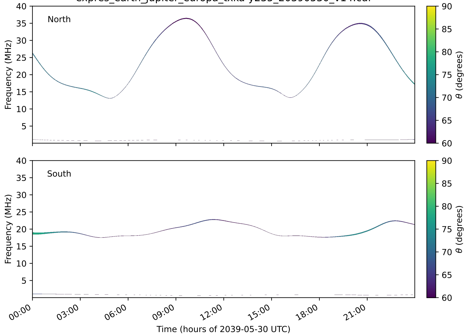
expres_earth_jupiter_europa_txka-y235_20390530_v14.cdf
