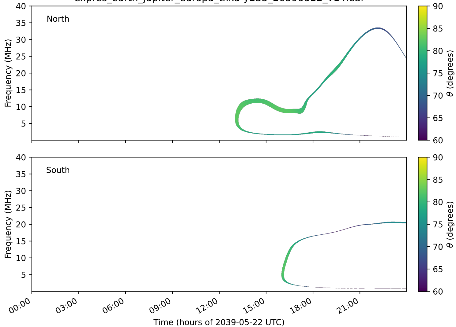
expres_earth_jupiter_europa_txka-y235_20390522_v14.cdf
