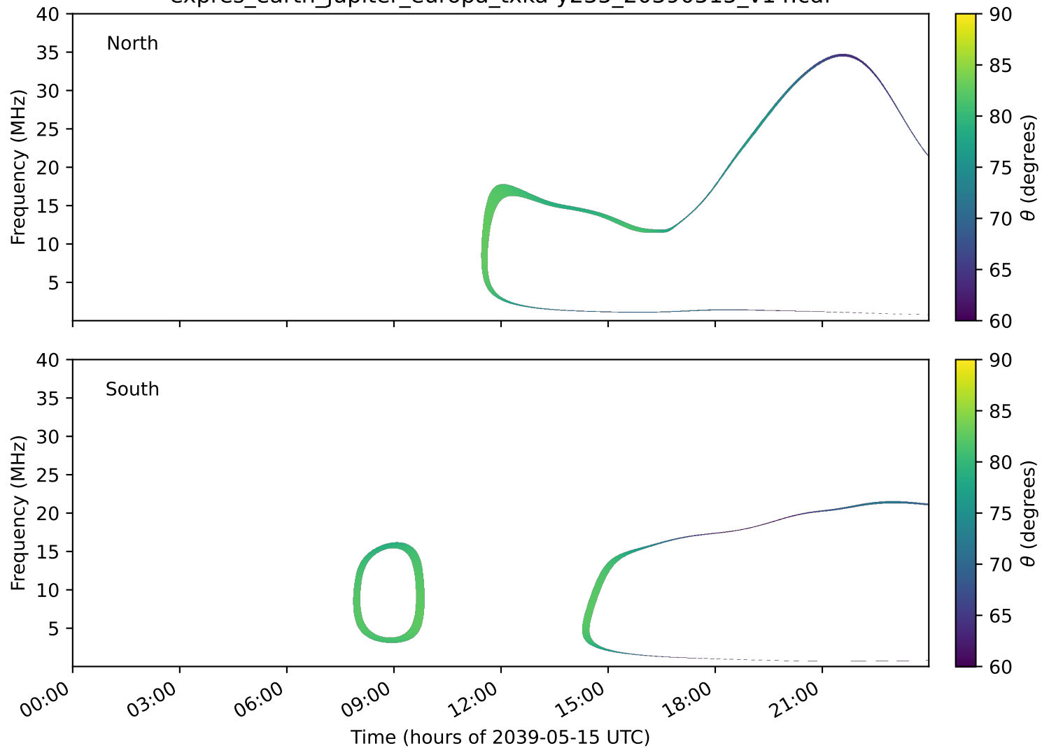
expres_earth_jupiter_europa_txka-y235_20390515_v14.cdf
