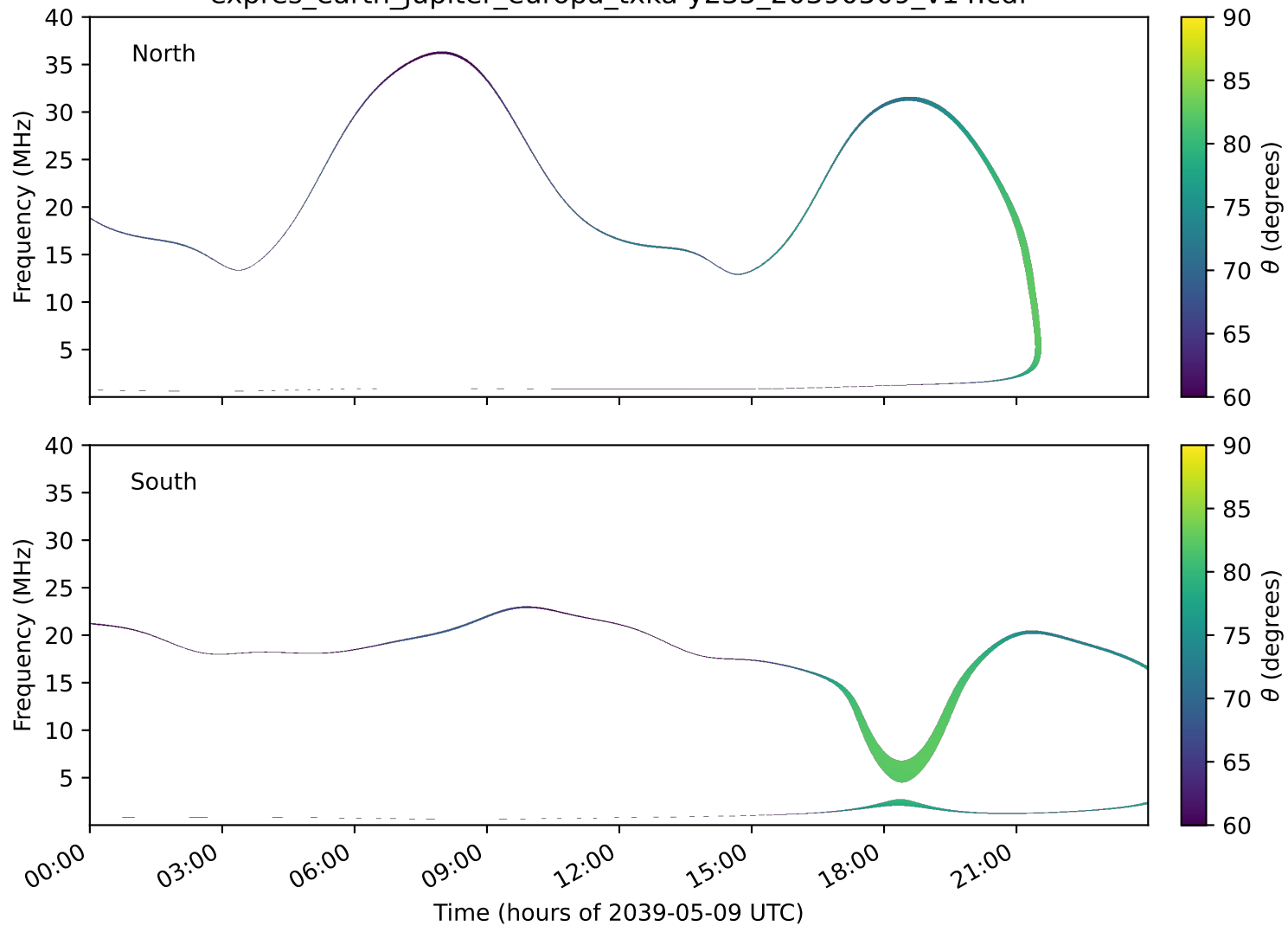
expres_earth_jupiter_europa_txka-y235_20390509_v14.cdf
