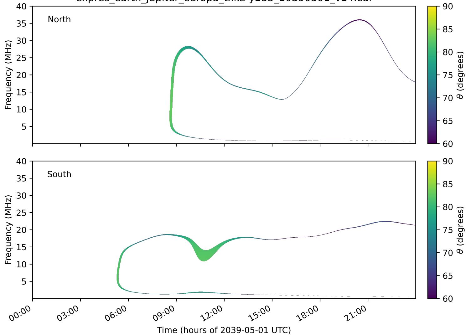
expres_earth_jupiter_europa_txka-y235_20390501_v14.cdf
