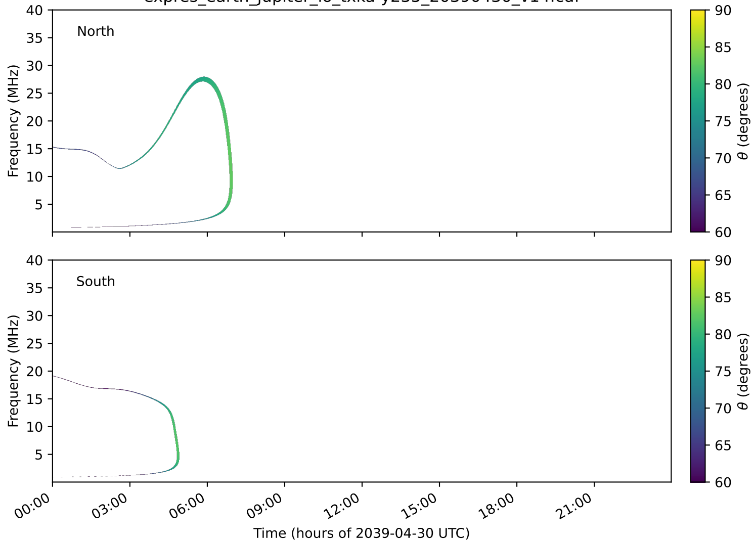
expres_earth_jupiter_io_txka-y235_20390430_v14.cdf
