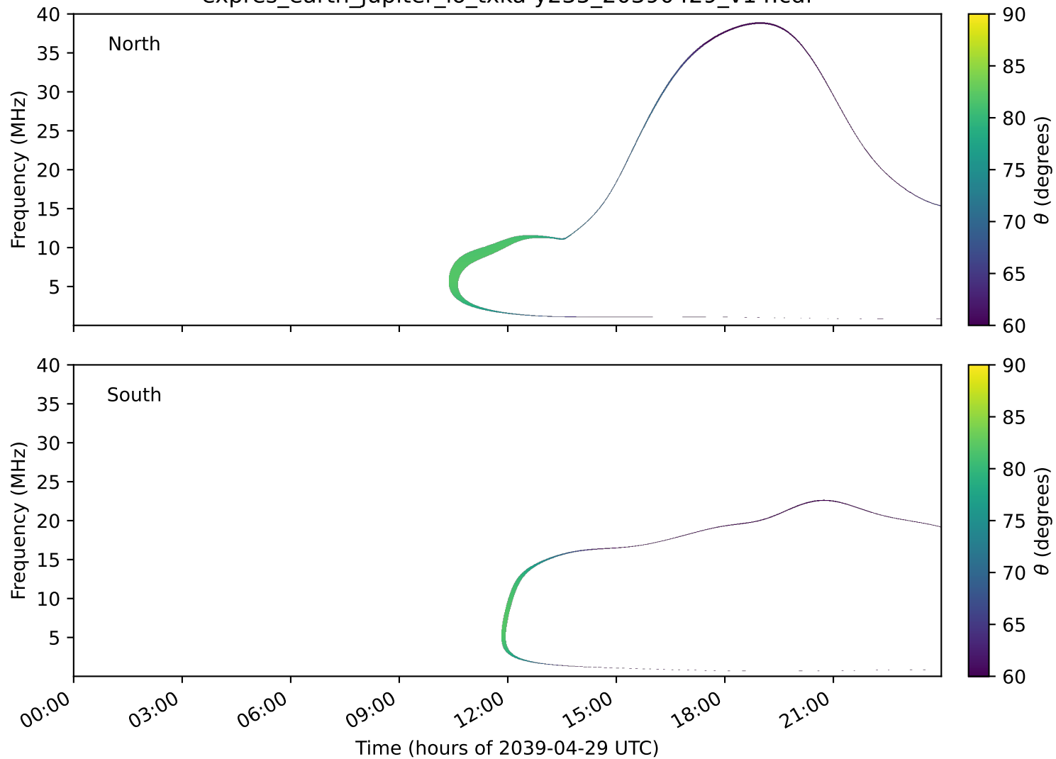
expres_earth_jupiter_io_txka-y235_20390429_v14.cdf
