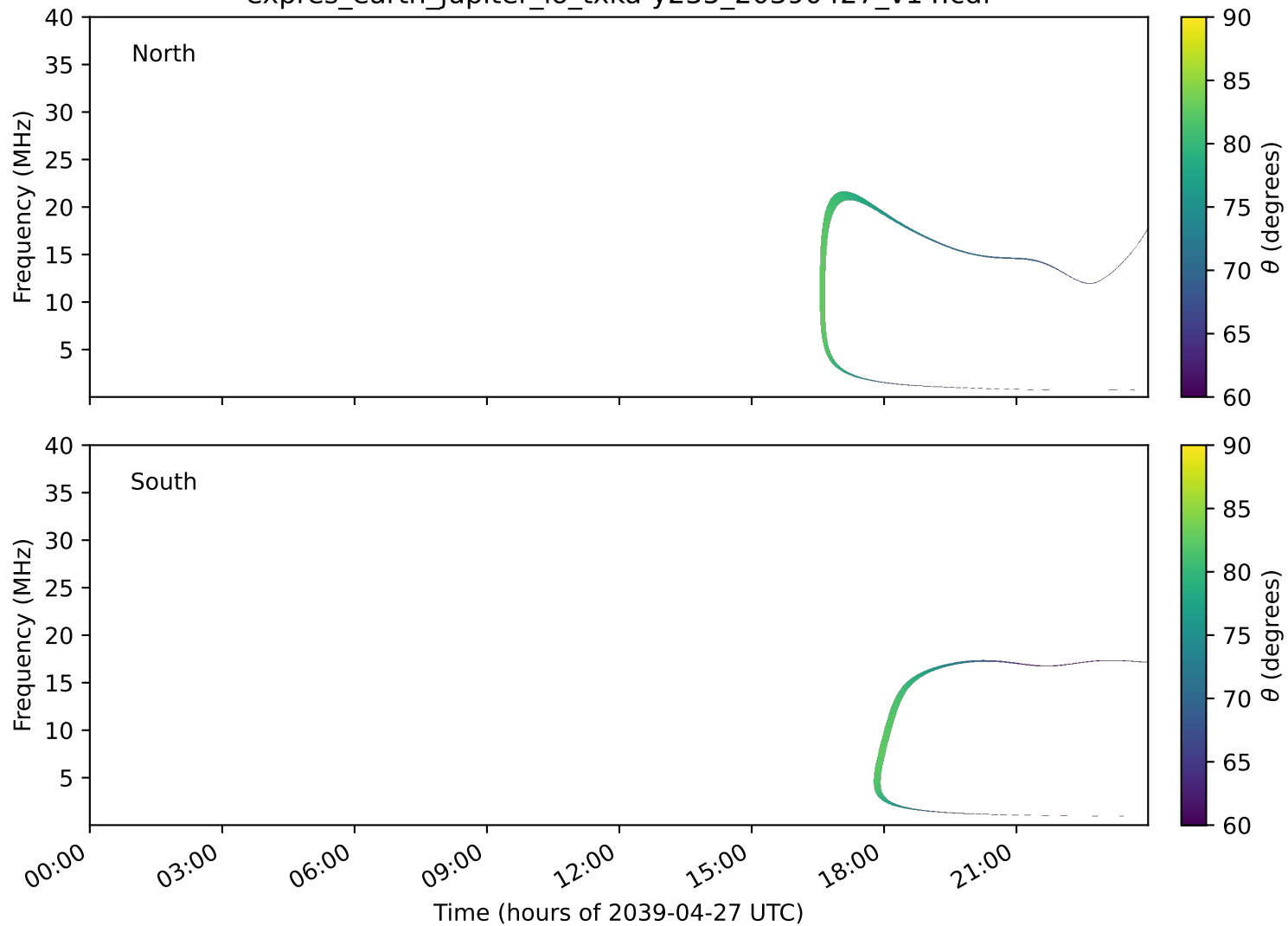
expres_earth_jupiter_io_txka-y235_20390427_v14.cdf
