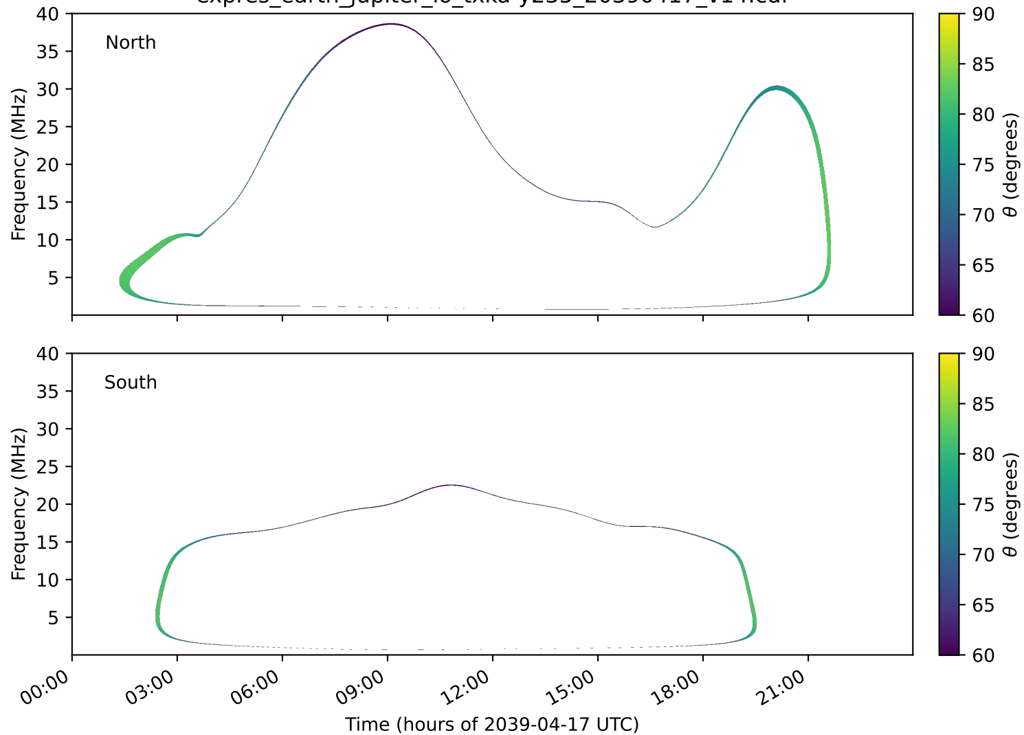
expres_earth_jupiter_io_txka-y235_20390417_v14.cdf
