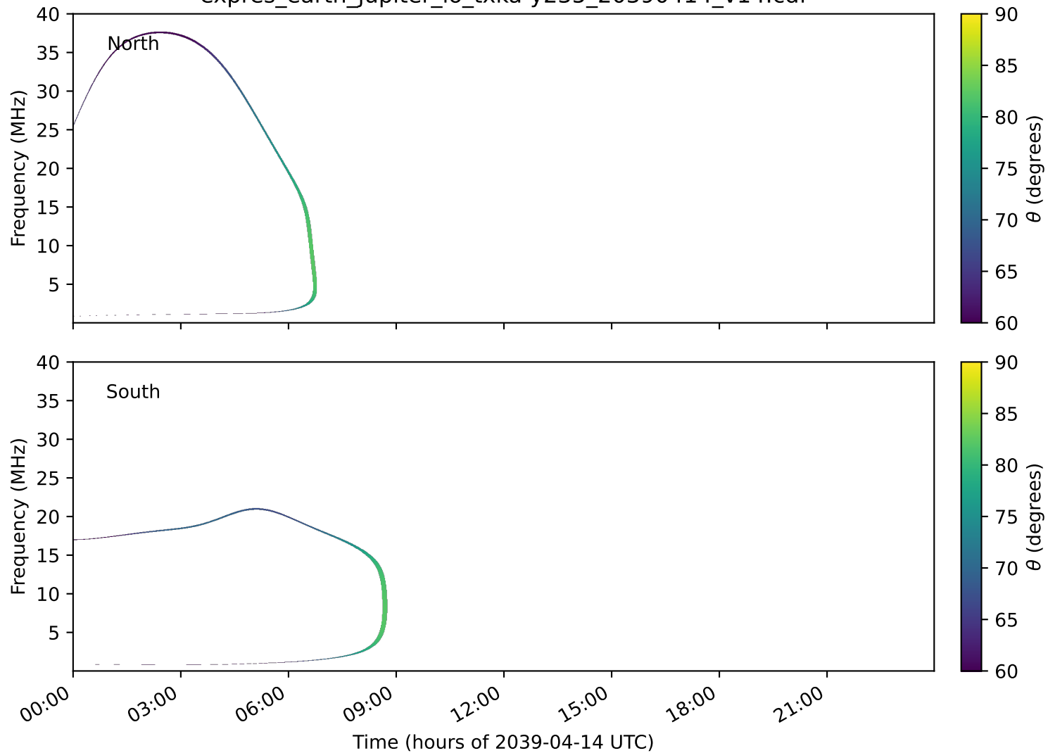
expres_earth_jupiter_io_txka-y235_20390414_v14.cdf
