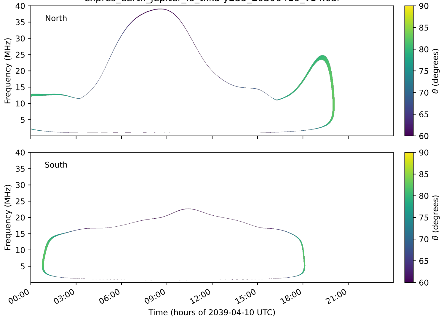
expres_earth_jupiter_io_txka-y235_20390410_v14.cdf
