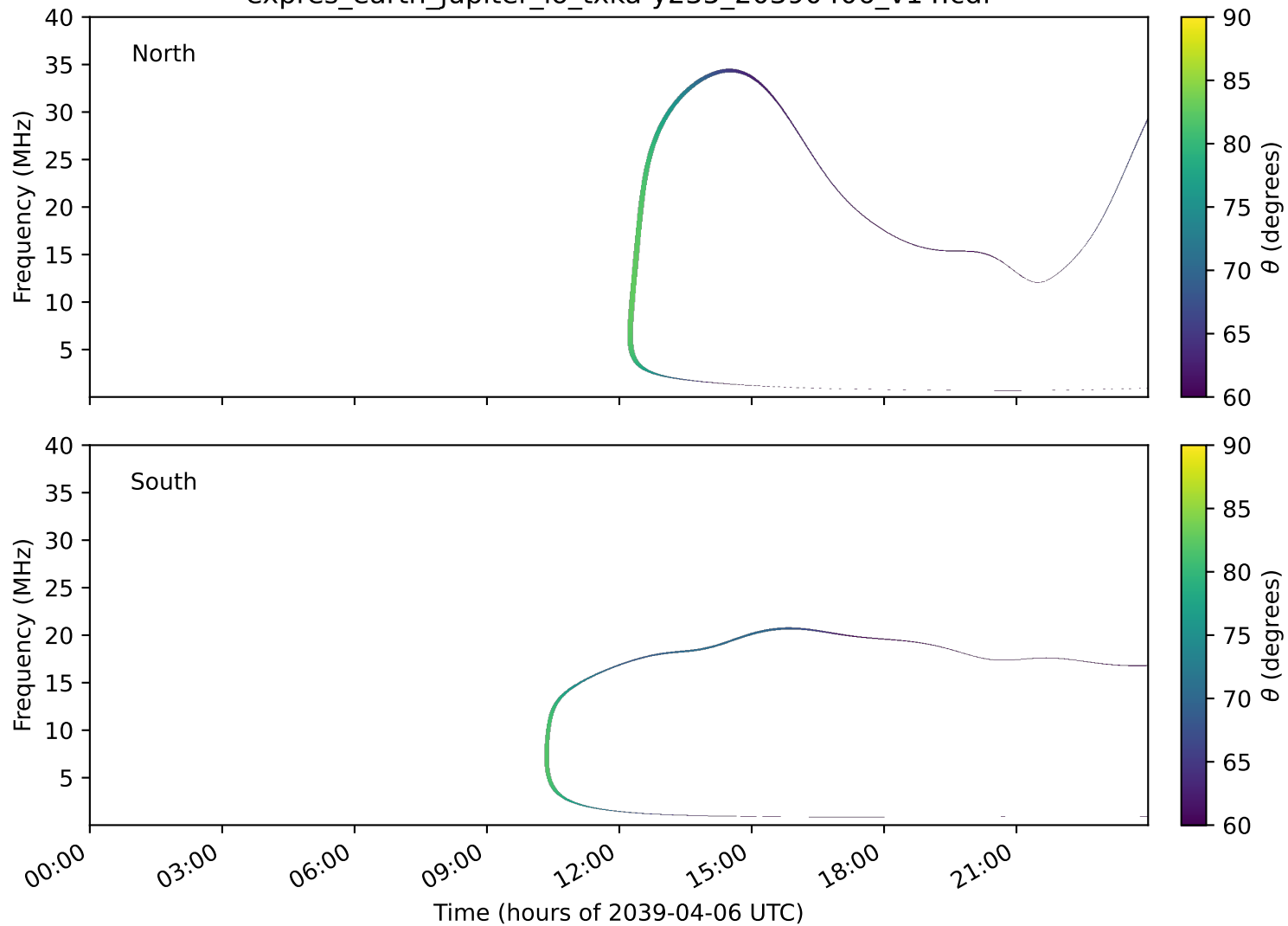
expres_earth_jupiter_io_txka-y235_20390406_v14.cdf
