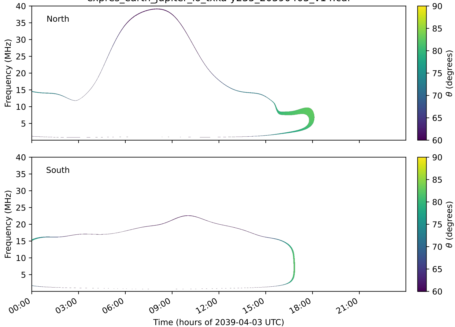
expres_earth_jupiter_io_txka-y235_20390403_v14.cdf
