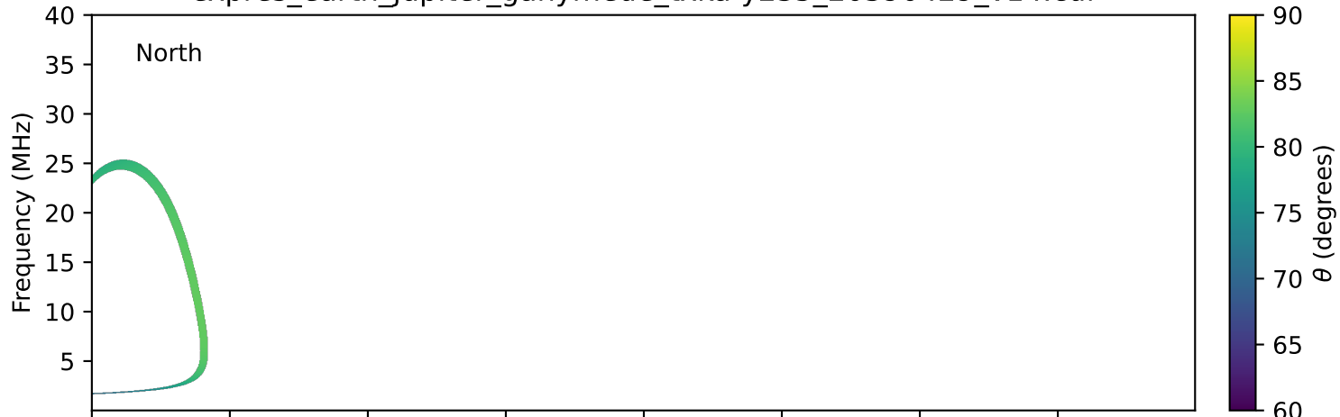
expres_earth_jupiter_ganymede_txka-y235_20390429_v14.cdf
