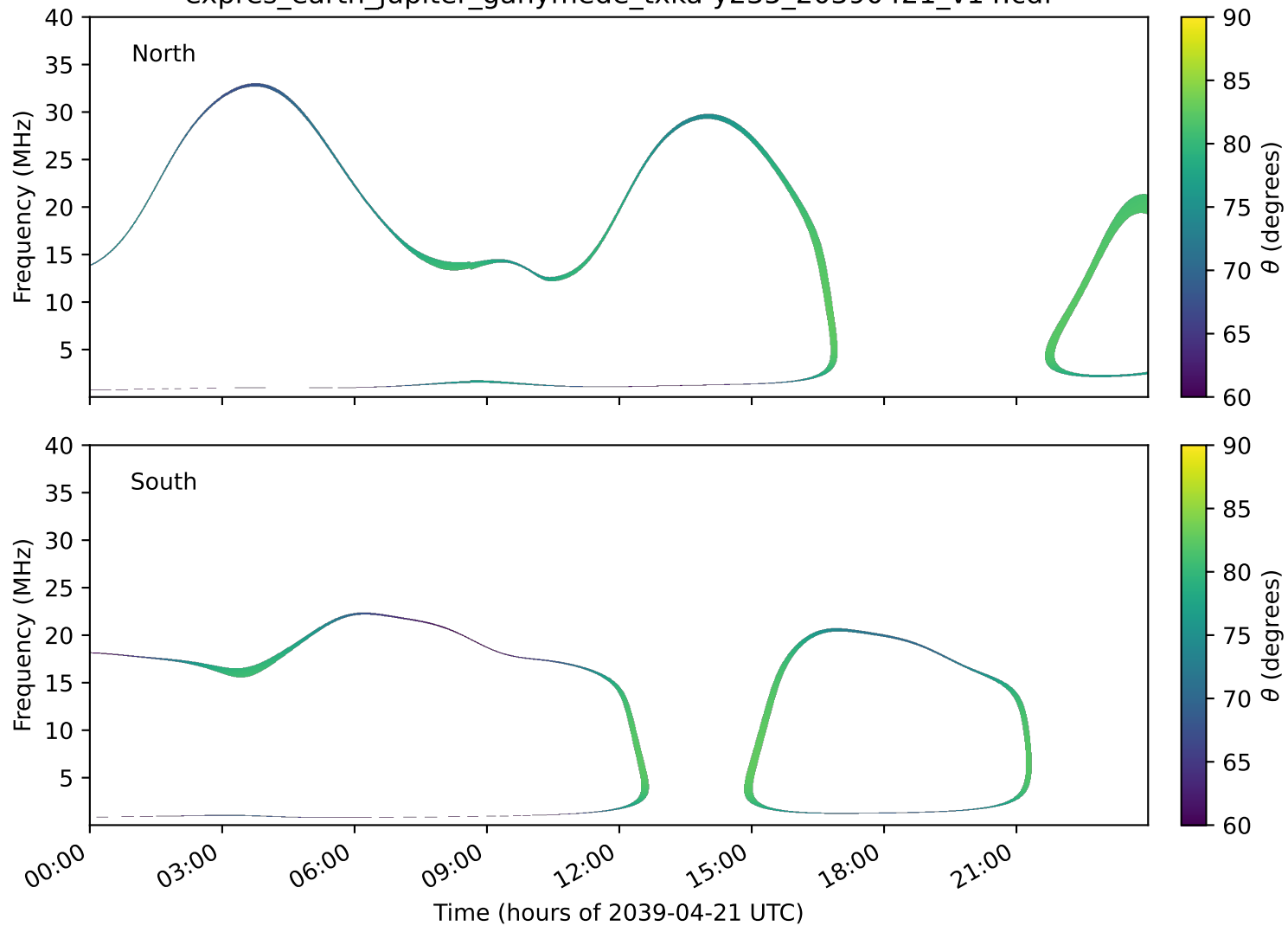
expres_earth_jupiter_ganymede_txka-y235_20390421_v14.cdf
