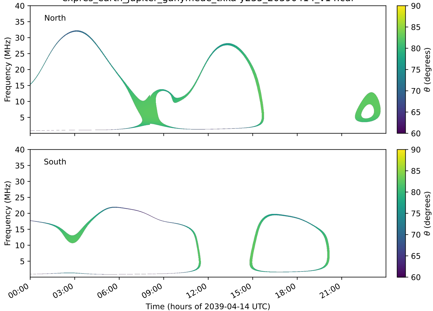
expres_earth_jupiter_ganymede_txka-y235_20390414_v14.cdf
