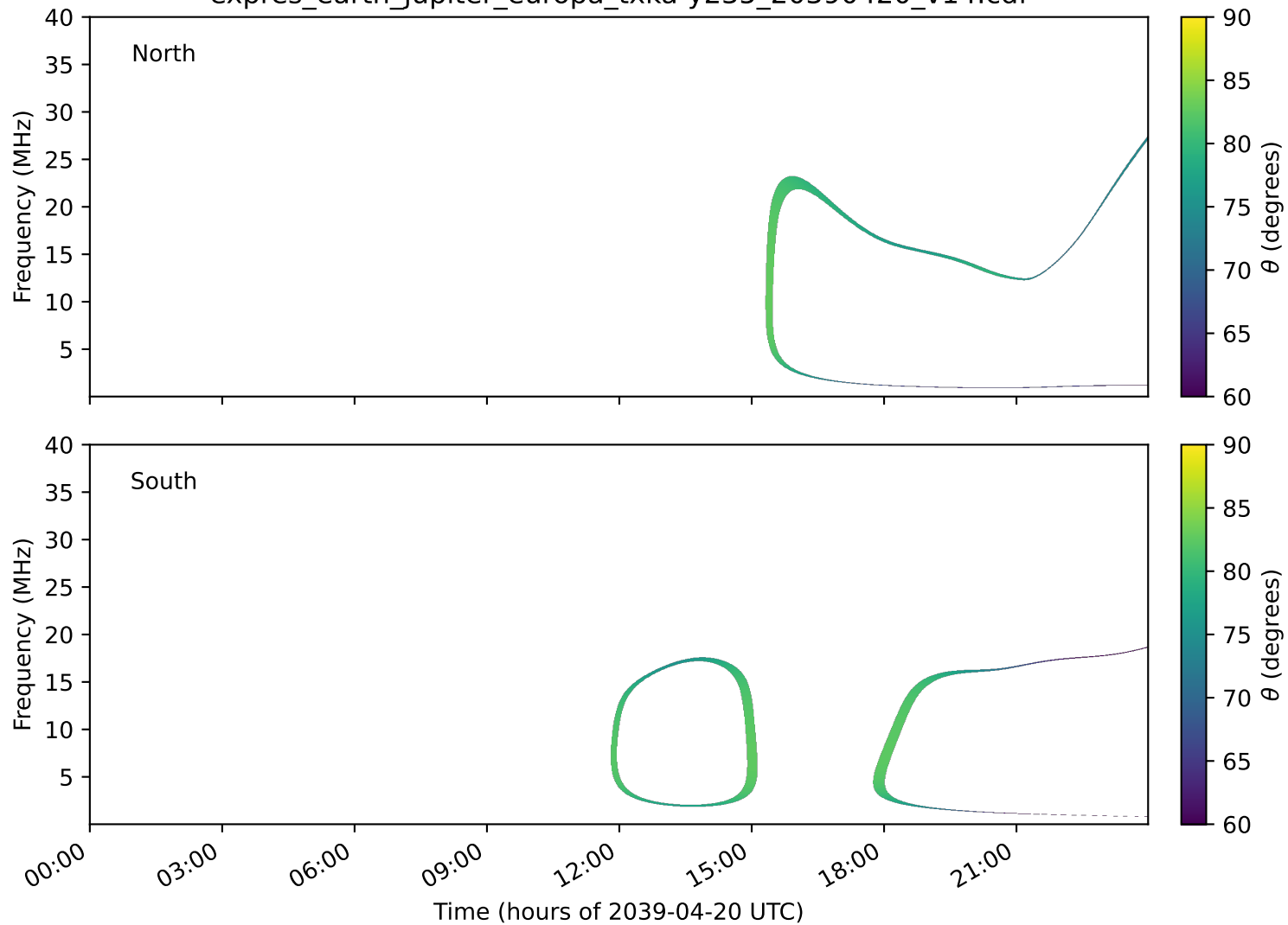
expres_earth_jupiter_europa_txka-y235_20390420_v14.cdf
