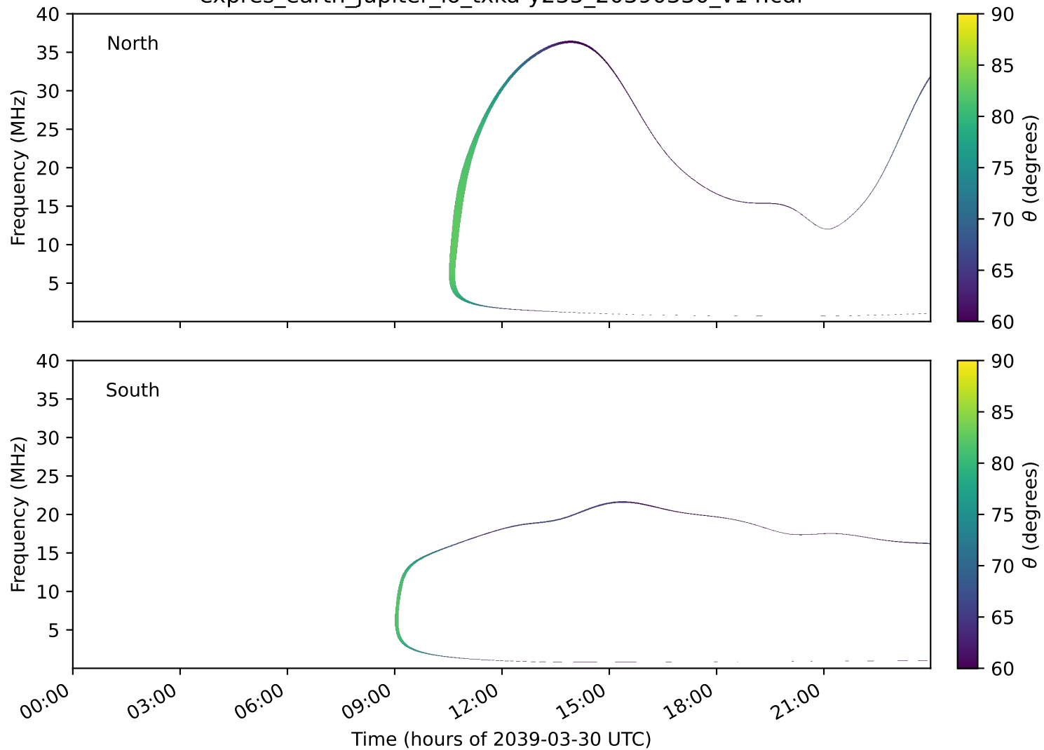
expres_earth_jupiter_io_txka-y235_20390330_v14.cdf
