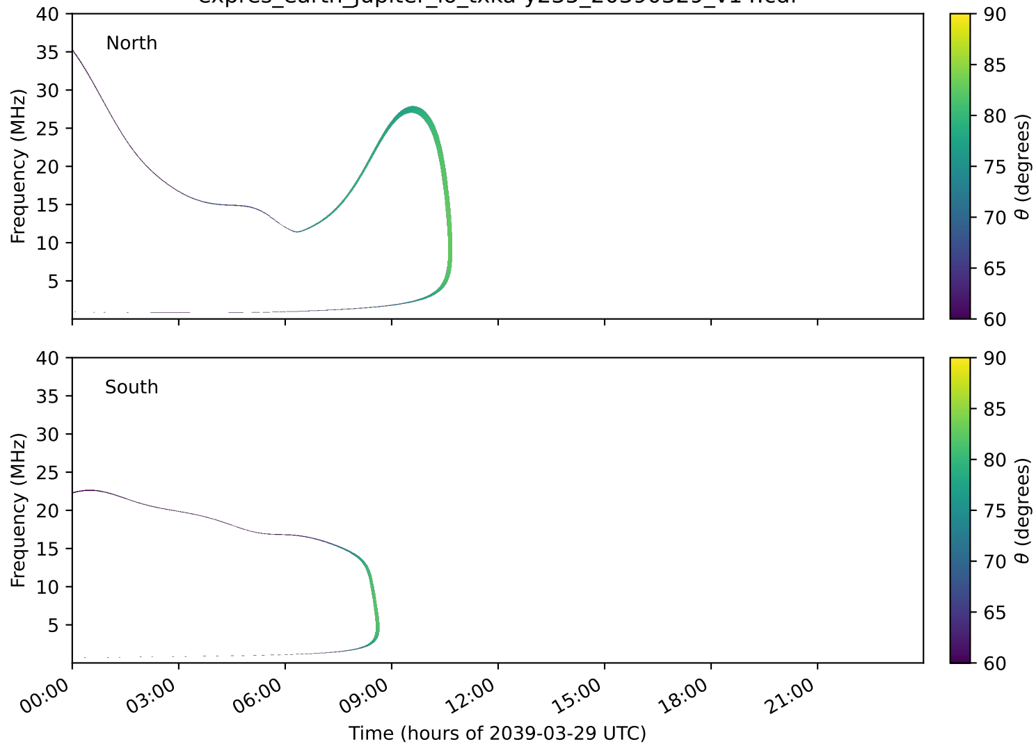
expres_earth_jupiter_io_txka-y235_20390329_v14.cdf
