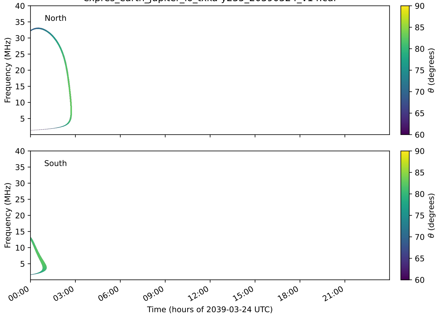
expres_earth_jupiter_io_txka-y235_20390324_v14.cdf
