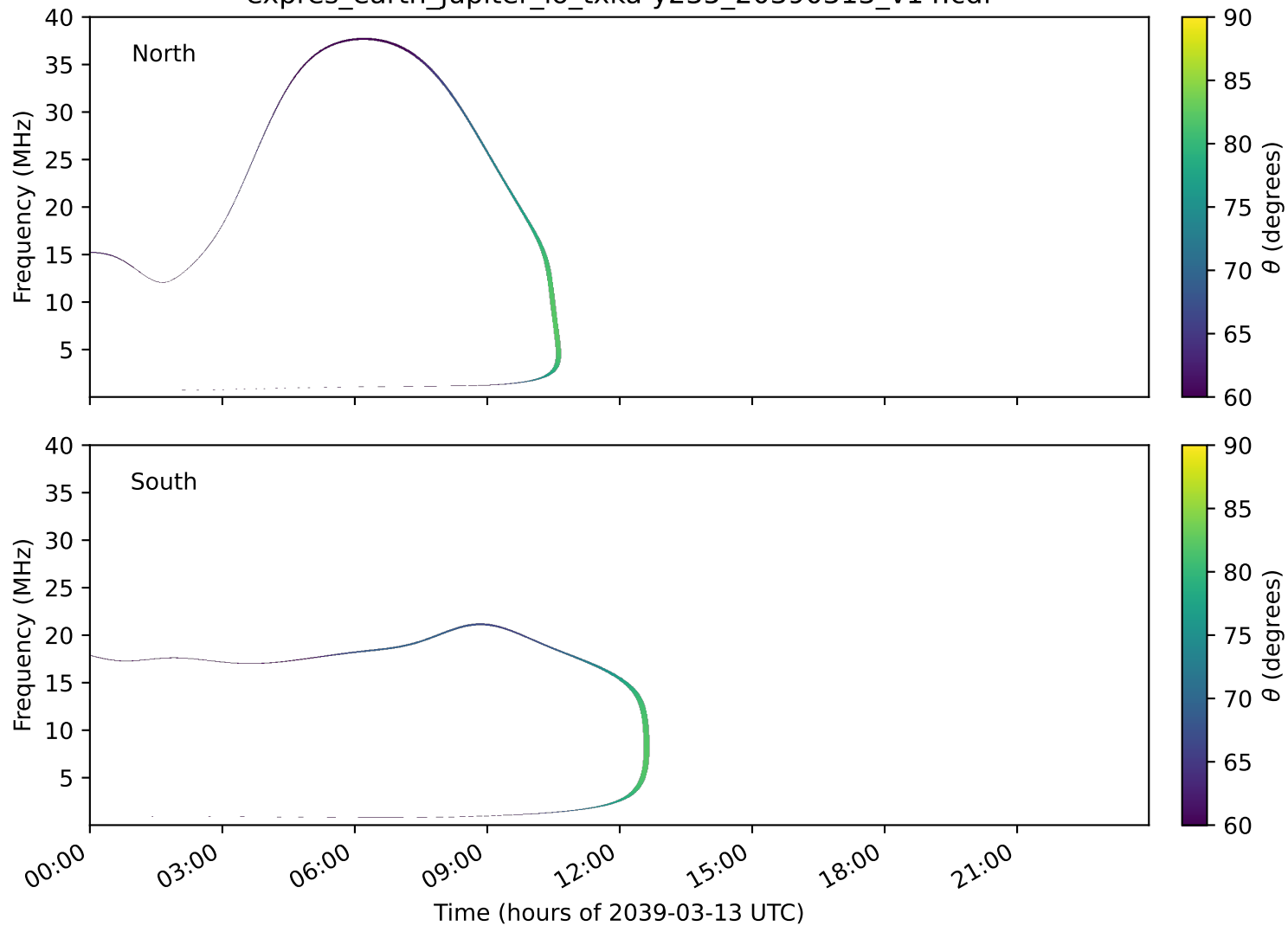
expres_earth_jupiter_io_txka-y235_20390313_v14.cdf
