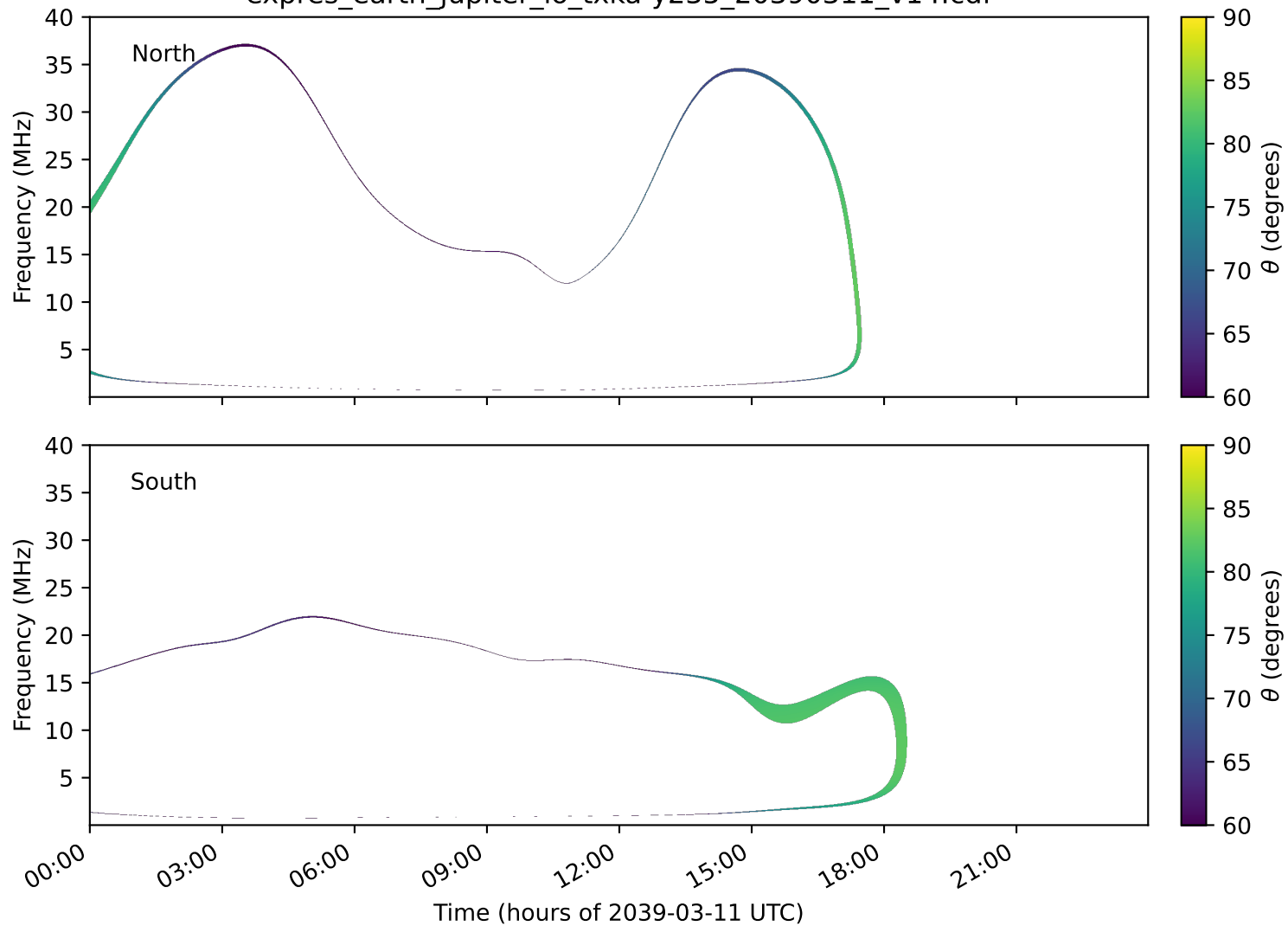
expres_earth_jupiter_io_txka-y235_20390311_v14.cdf
