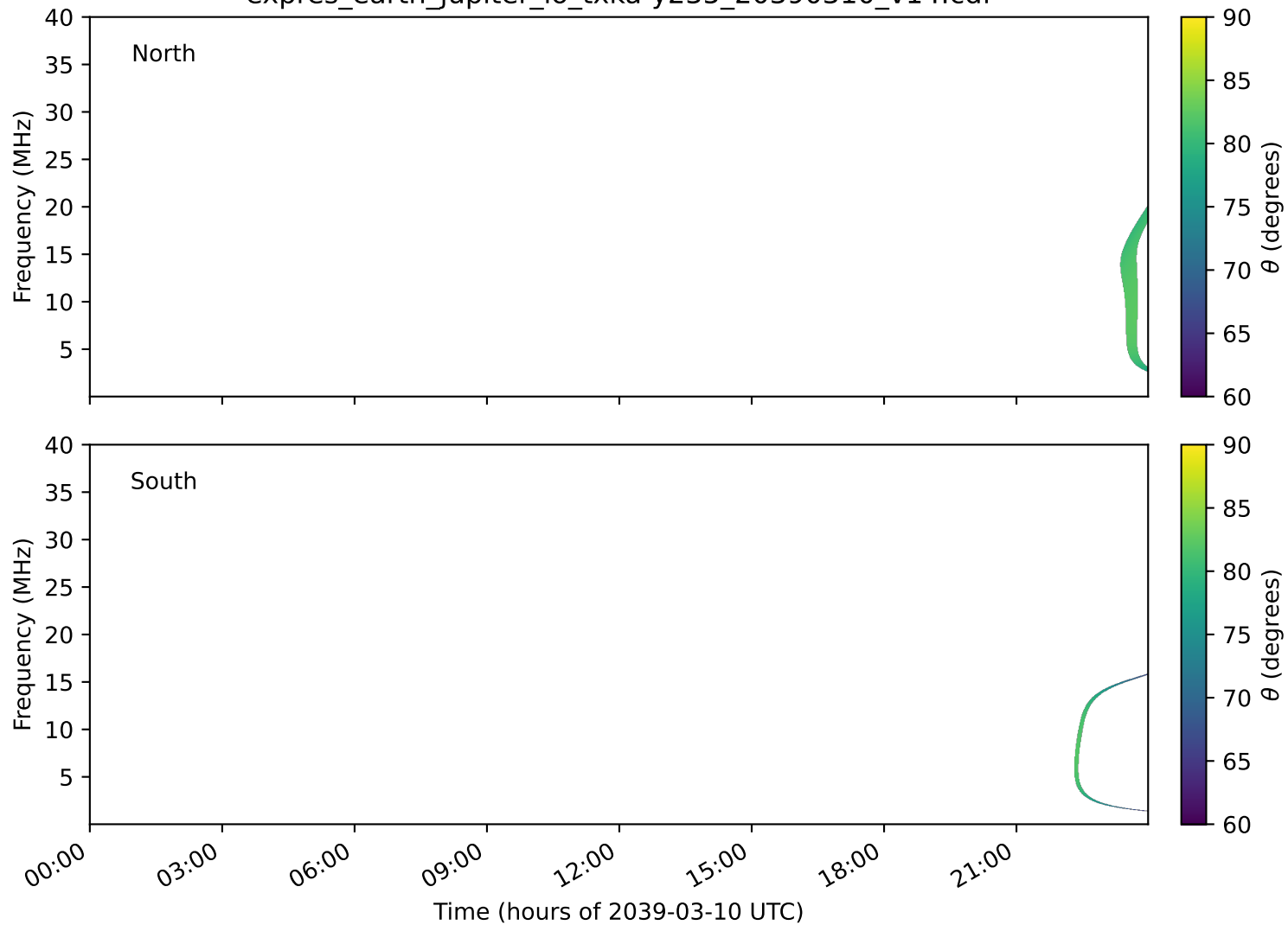
expres_earth_jupiter_io_txka-y235_20390310_v14.cdf
