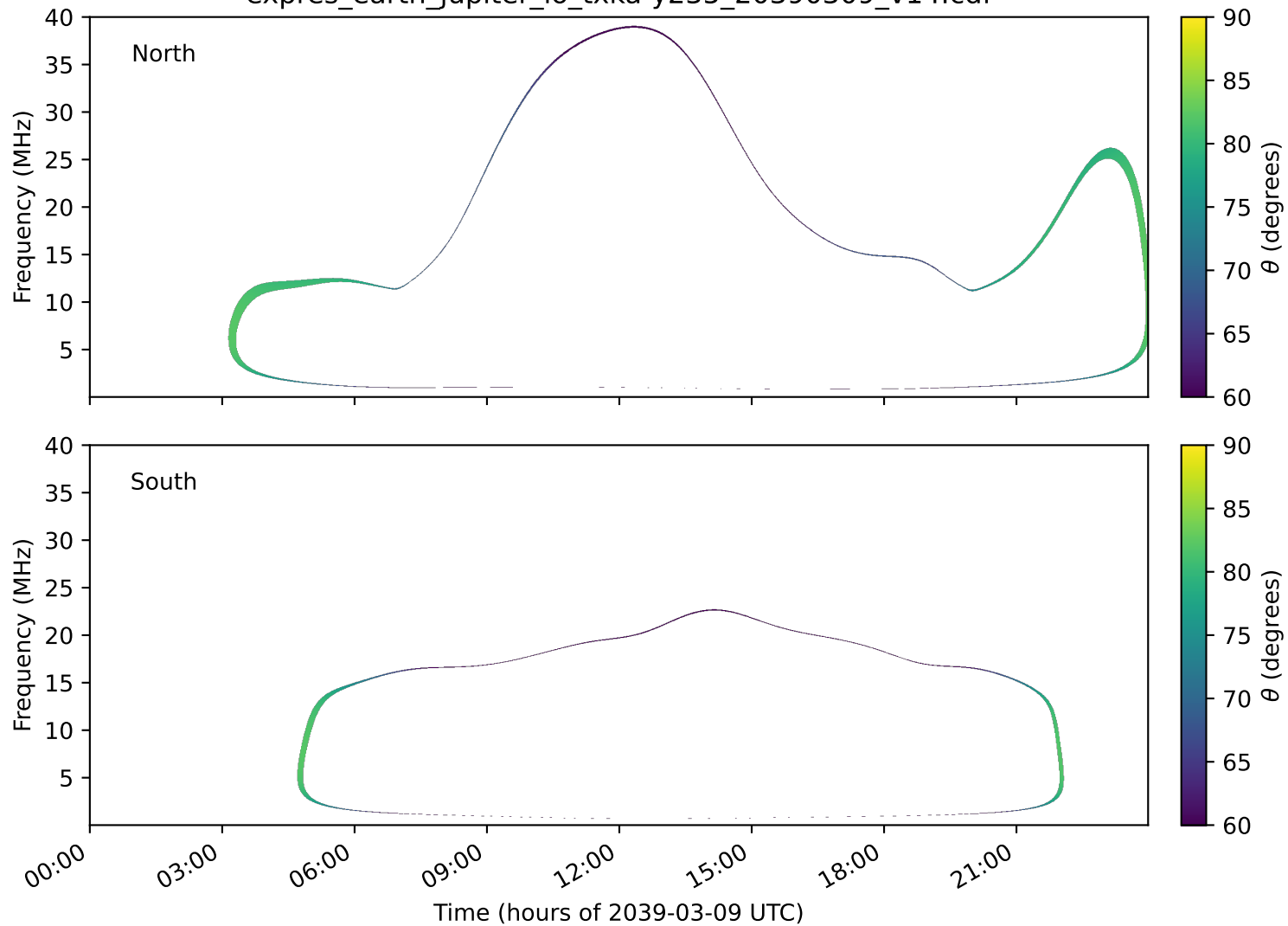
expres_earth_jupiter_io_txka-y235_20390309_v14.cdf
