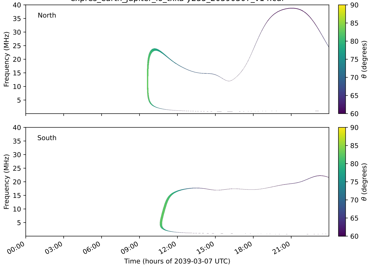
expres_earth_jupiter_io_txka-y235_20390307_v14.cdf
