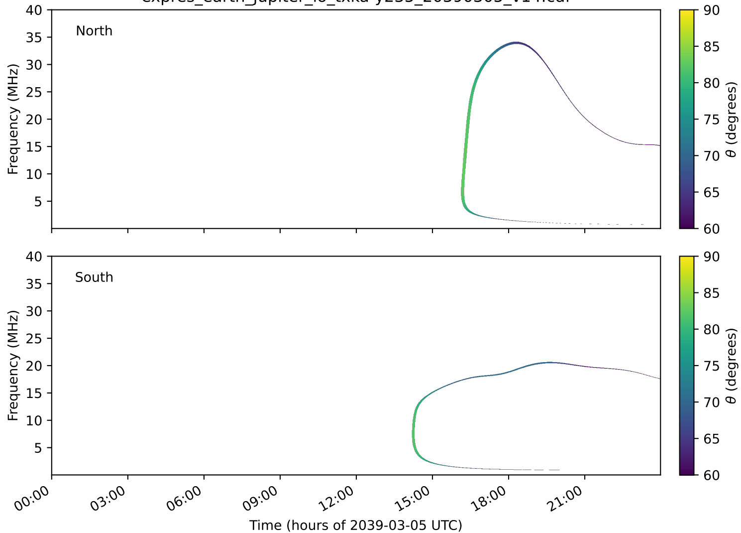
expres_earth_jupiter_io_txka-y235_20390305_v14.cdf
