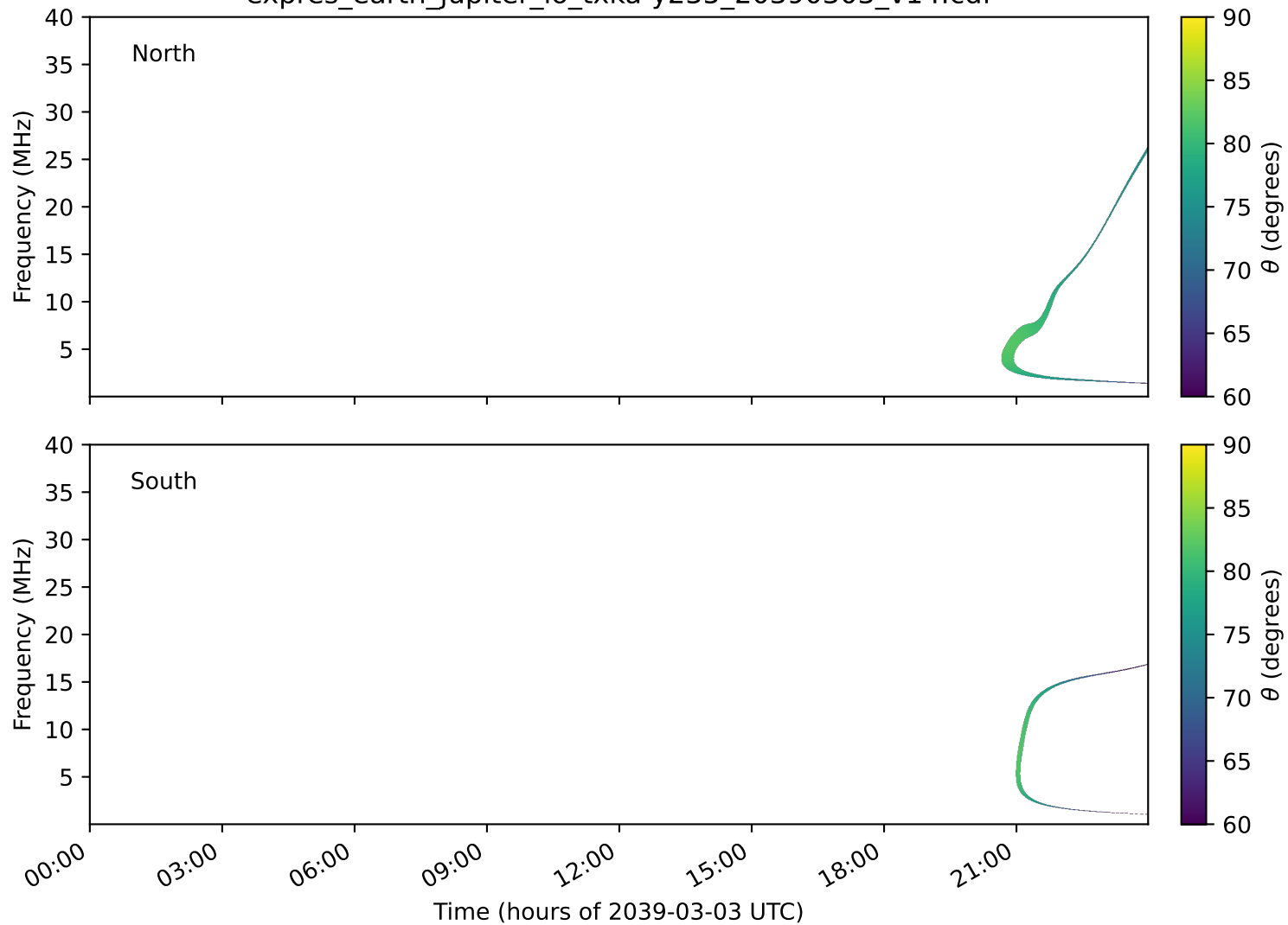
expres_earth_jupiter_io_txka-y235_20390303_v14.cdf
