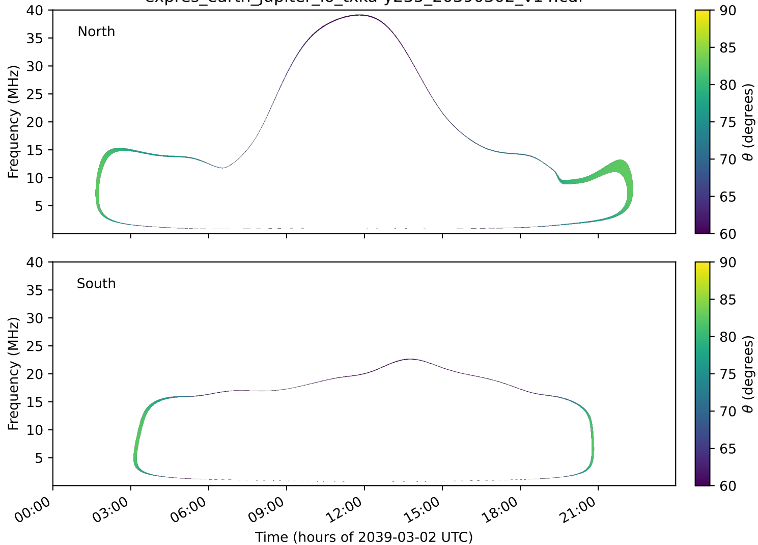
expres_earth_jupiter_io_txka-y235_20390302_v14.cdf
