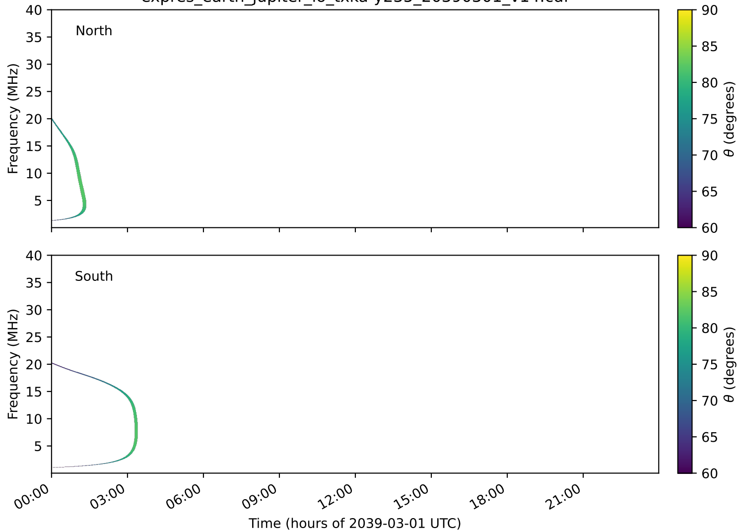
expres_earth_jupiter_io_txka-y235_20390301_v14.cdf
