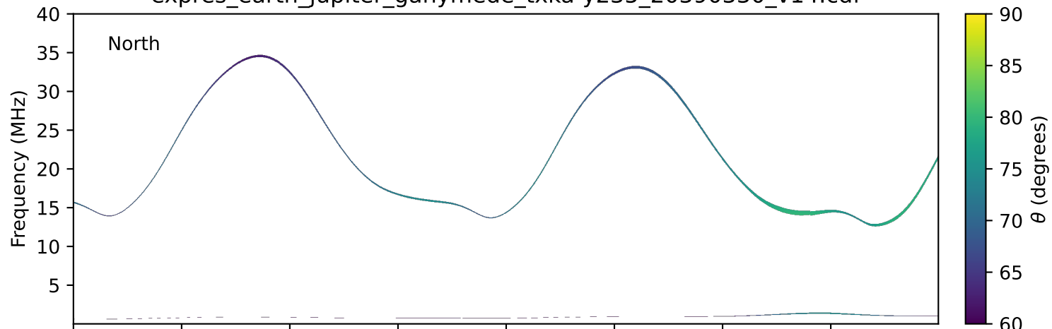
expres_earth_jupiter_ganymede_txka-y235_20390330_v14.cdf
