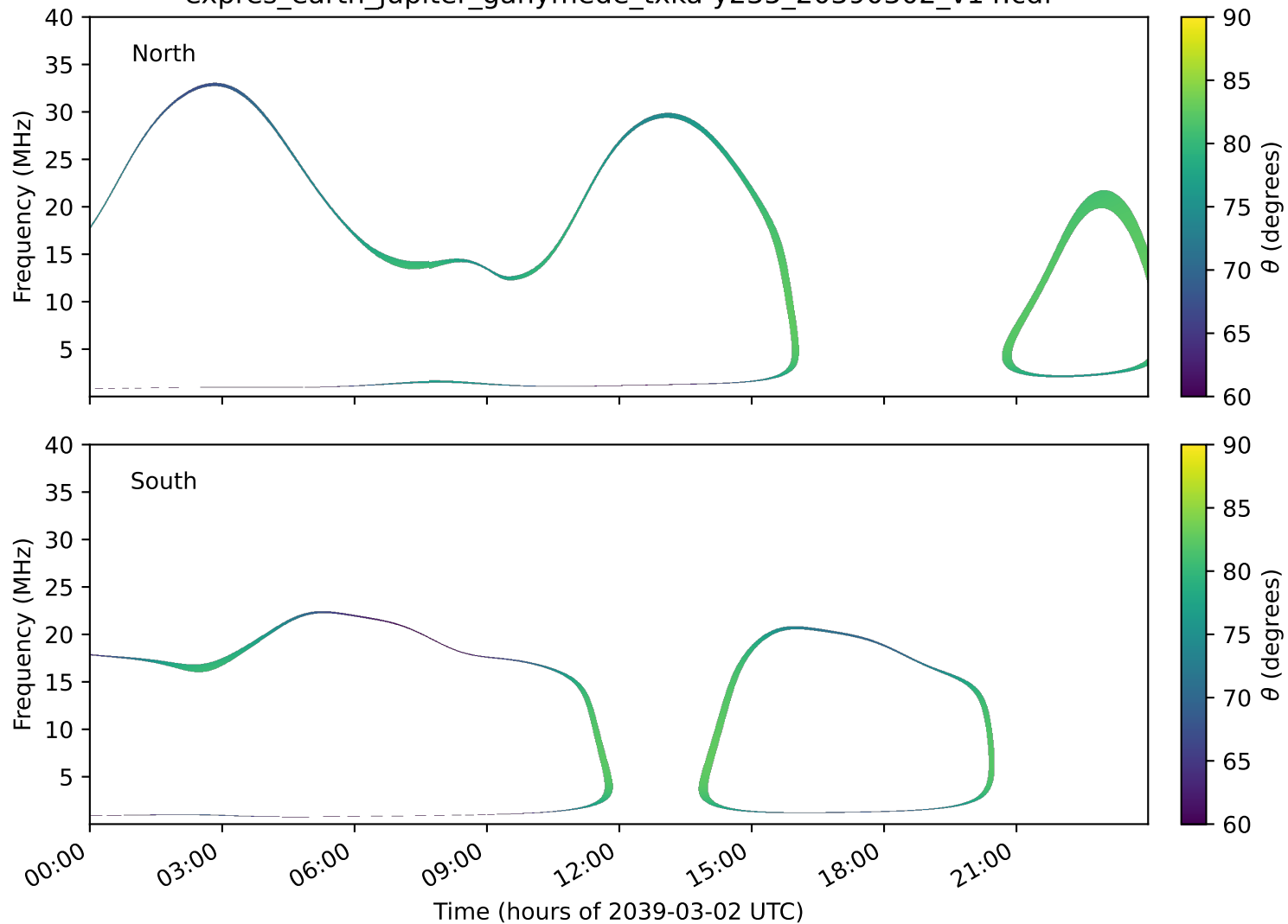
expres_earth_jupiter_ganymede_txka-y235_20390302_v14.cdf
