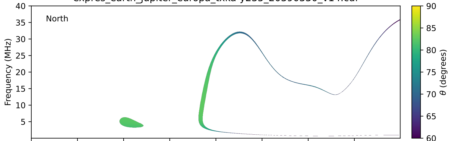
expres_earth_jupiter_europa_txka-y235_20390330_v14.cdf
