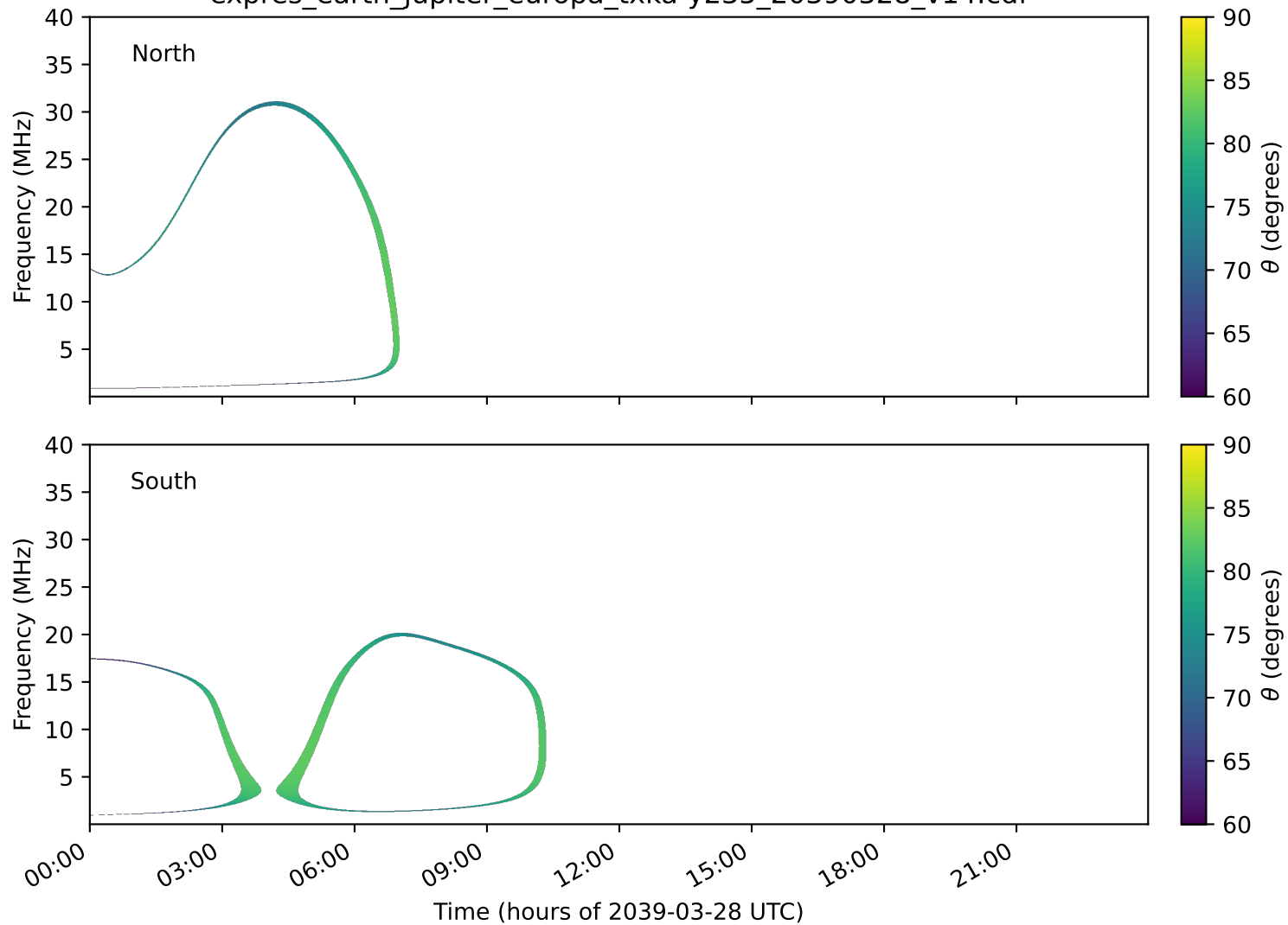
expres_earth_jupiter_europa_txka-y235_20390328_v14.cdf
