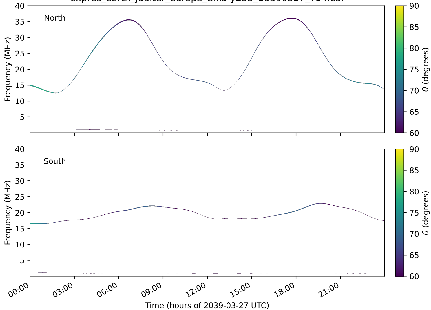
expres_earth_jupiter_europa_txka-y235_20390327_v14.cdf
