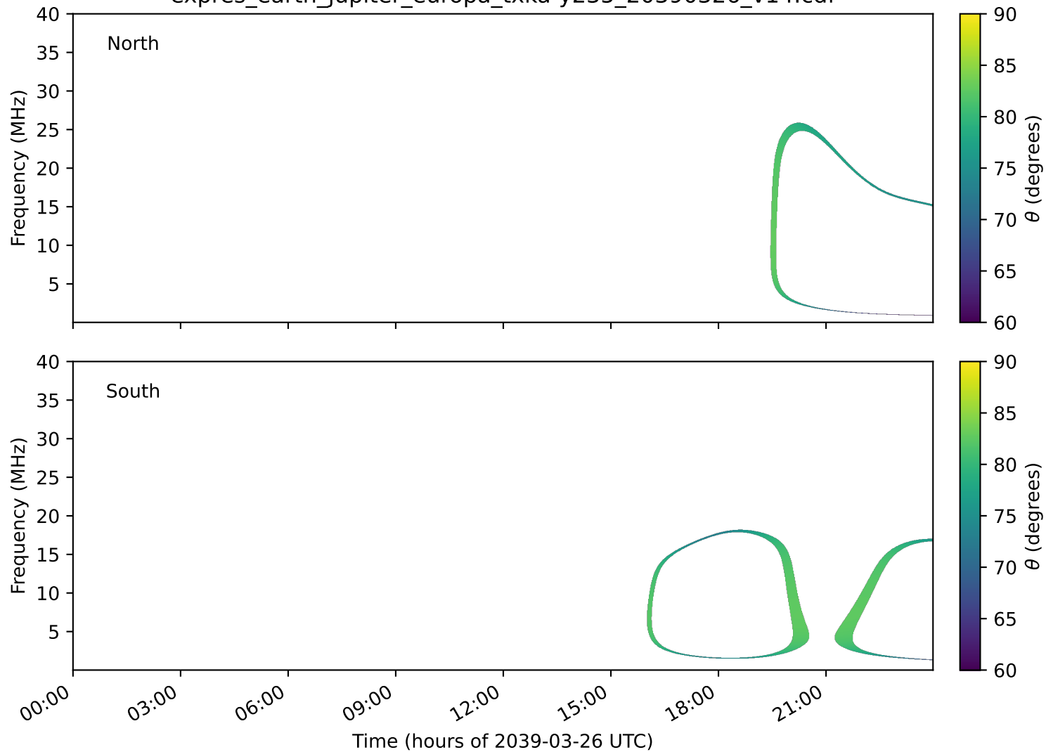
expres_earth_jupiter_europa_txka-y235_20390326_v14.cdf
