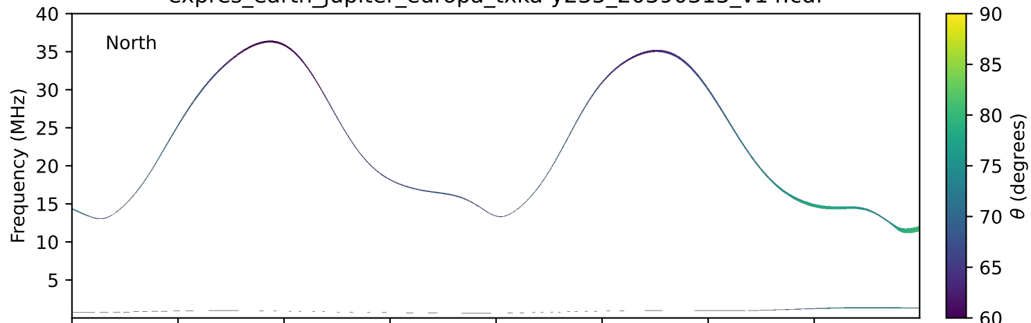
expres_earth_jupiter_europa_txka-y235_20390313_v14.cdf
